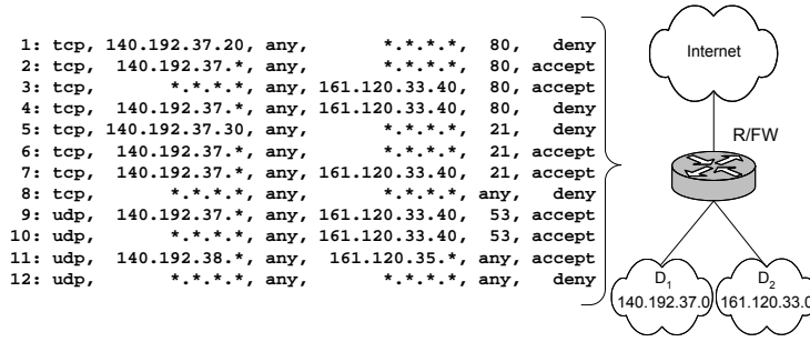
Fig. 1. An example for centralized firewall setup.
